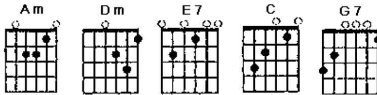
Chord diagram Am, Dm, E7 plus C, and G7
